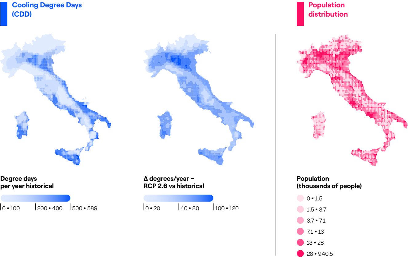
Cooling Degree Days (CDDs) in the 1990–2020 period and the expected change in the RCP 2.6 scenario. On the right, the figure shows the population distribution (1990–2020) for the same nodes of the climate models, indicating the more heavily populated areas, which have a greater weight in calculating the metric at the country level.
